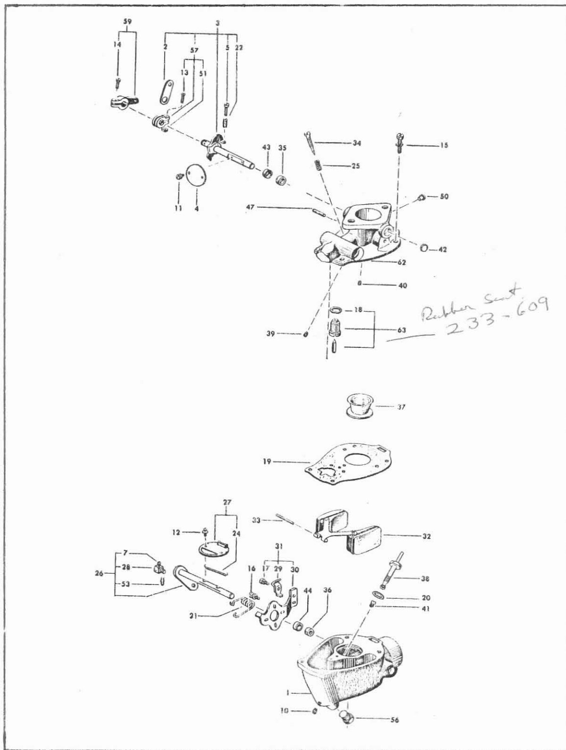
TSX-514 EXPLODED VIEW PARTS LIST ON REVERSE SIDE
