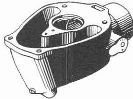
CARBURETOR BODY ASSY
